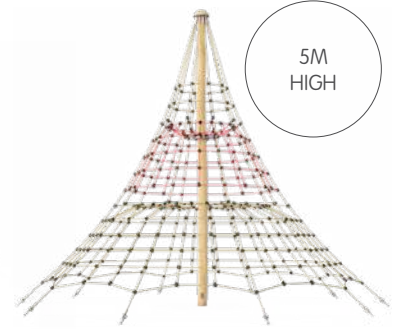
Tree Climber NRO834
